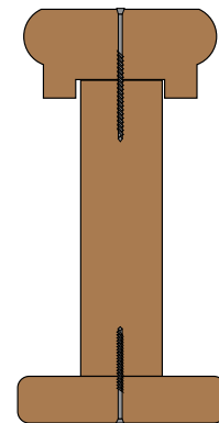
Handrail Diagram
